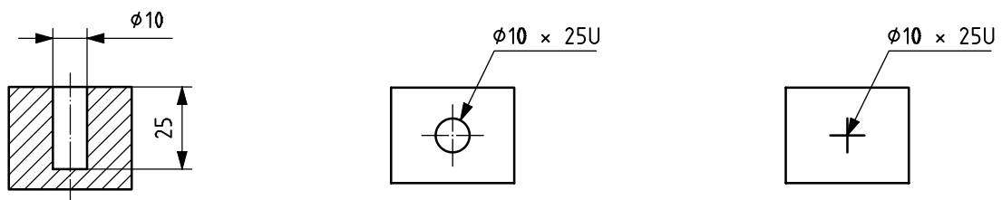
a) Complete representation and complete dimensioning
