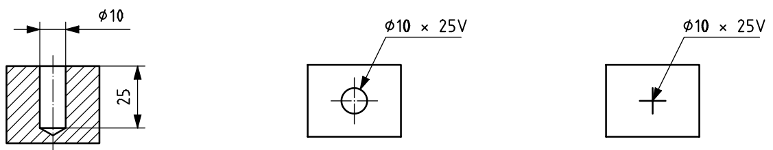
a) Complete representation and complete dimensioning
