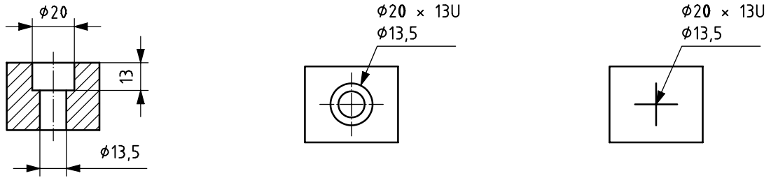
a) Complete representation and complete dimensioning
